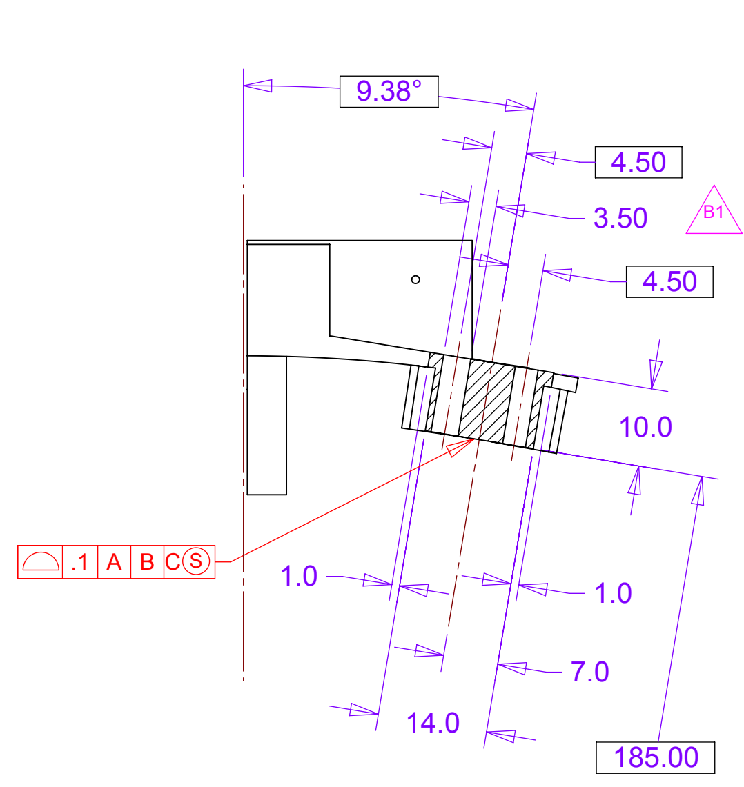
SECTION B-B
