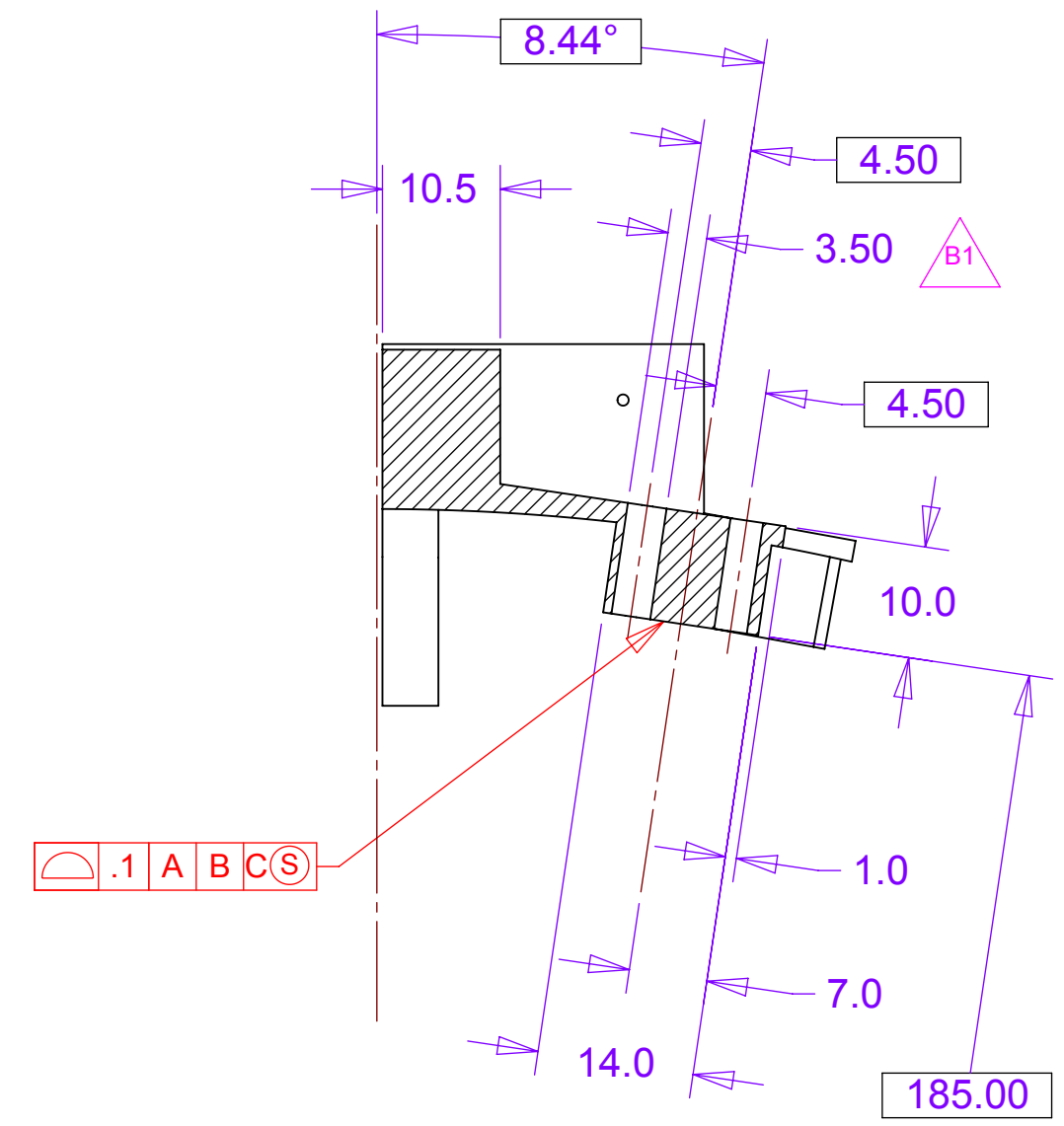
SECTION C-C
